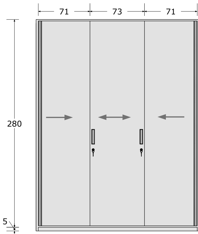
VISTA FRONTAL
