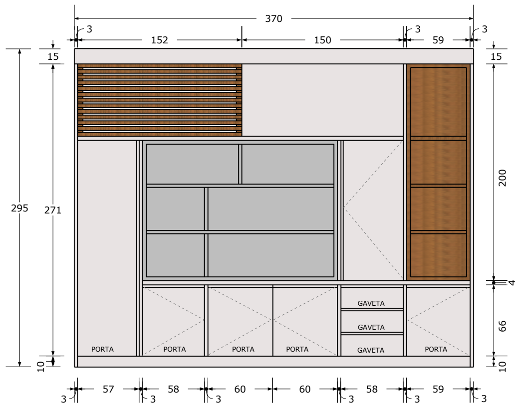
VISTA FRONTAL
