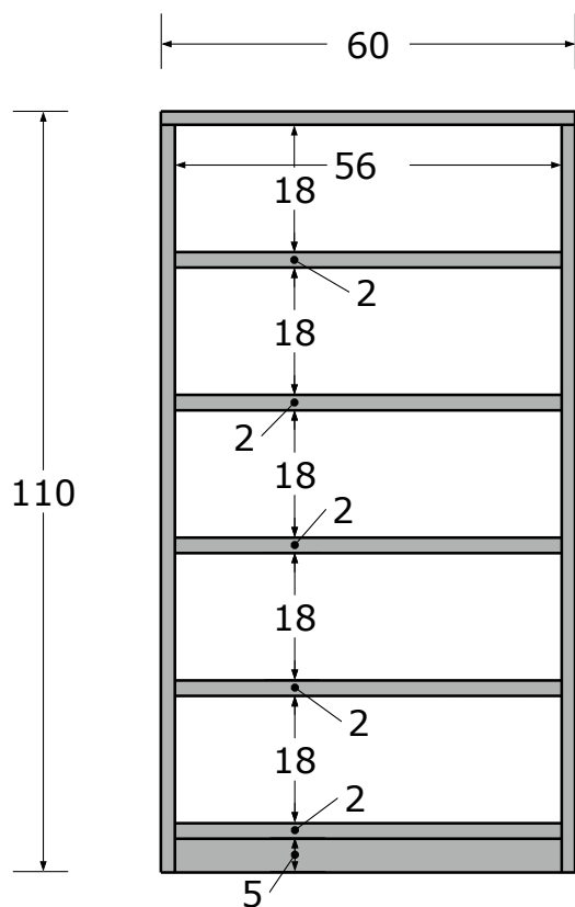
VISTA FRONTAL
