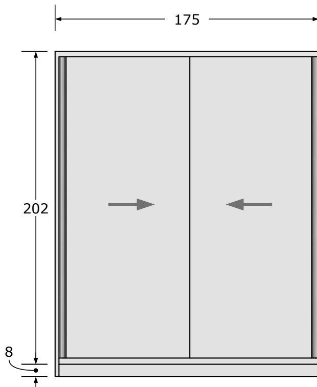
VISTA FRONTAL
