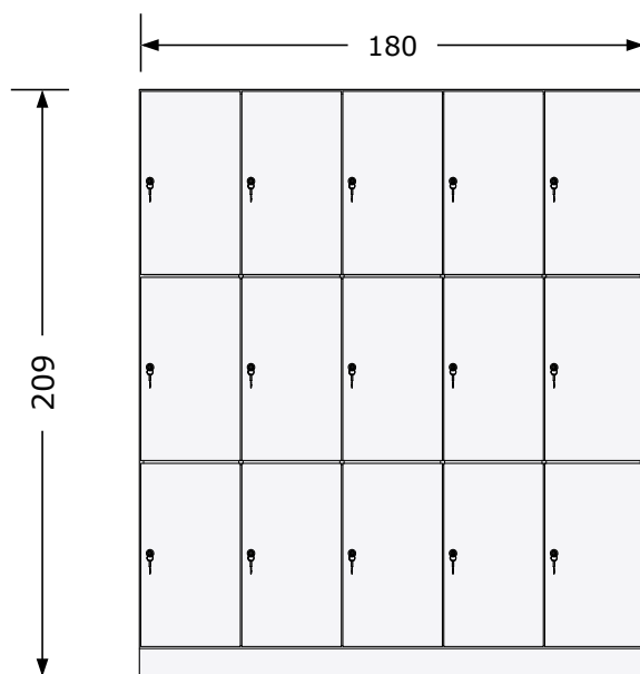
VISTA FRONTAL
