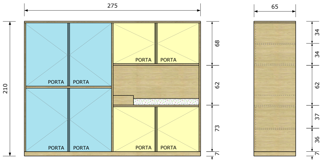
VISTA FRONTAL
