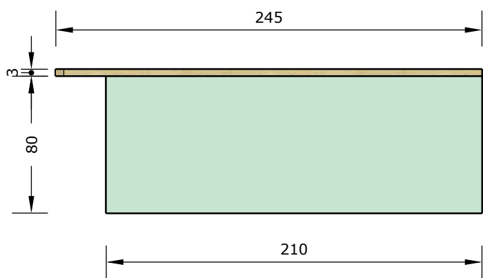
VISTA FRONTAL
