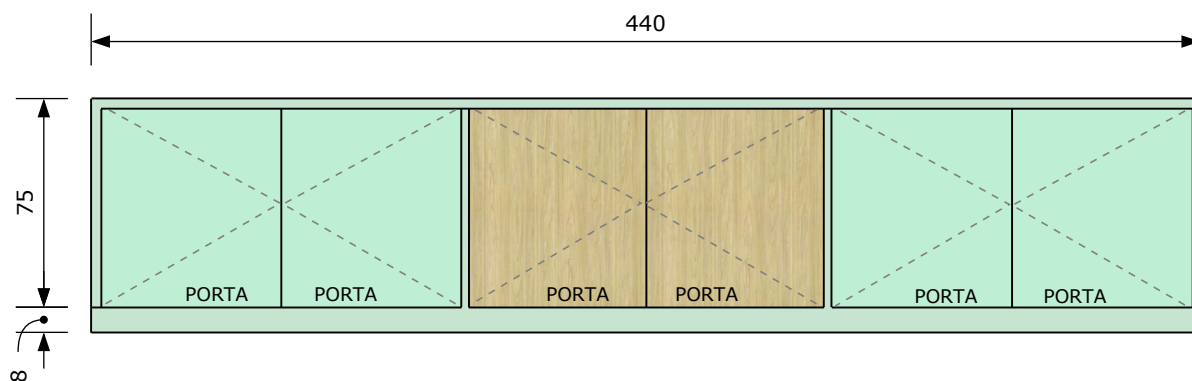
VISTA FRONTAL
